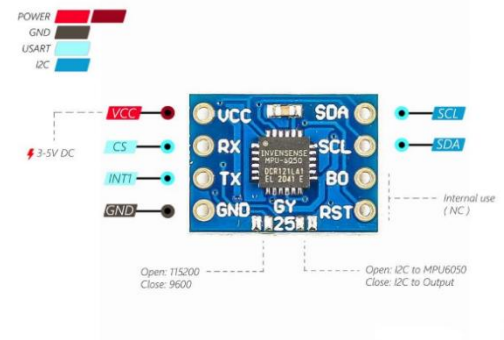
GY-25 Pinout
